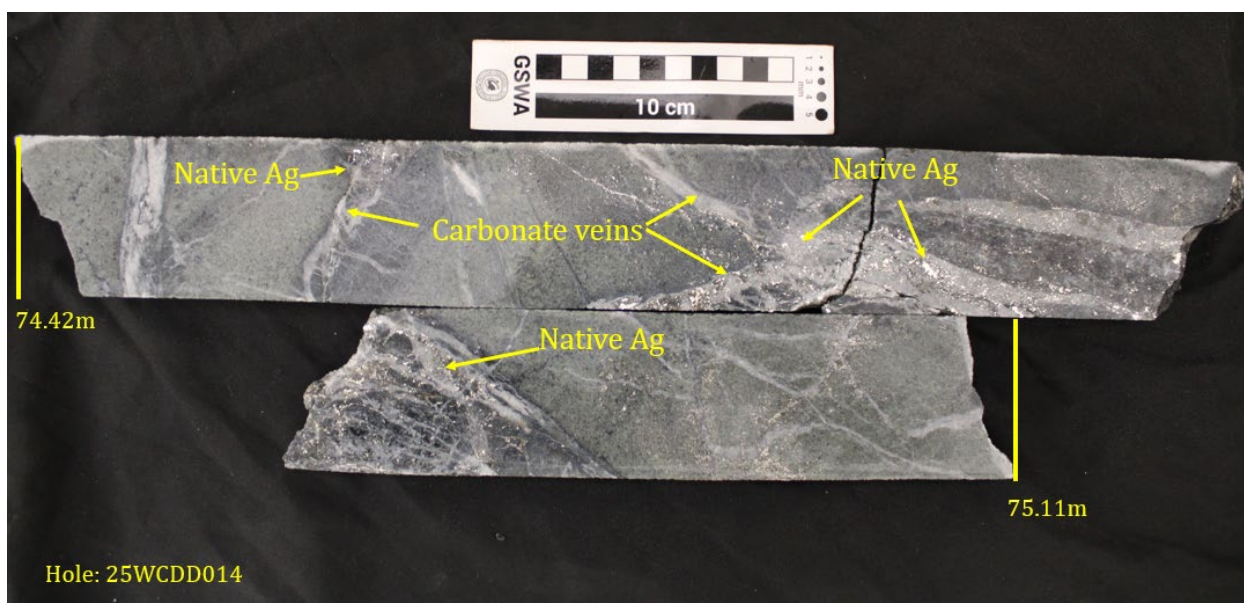
Photo 4: Photograph of cut half HQ3 drill core (25WCDD014) from 74.42m to 75.11m showing 1% visually estimated, 2mm to 4mm long native silver grains hosted within and adjacent to 1cm to 3cm thick carbonate veins in an ultramafic host rock.
